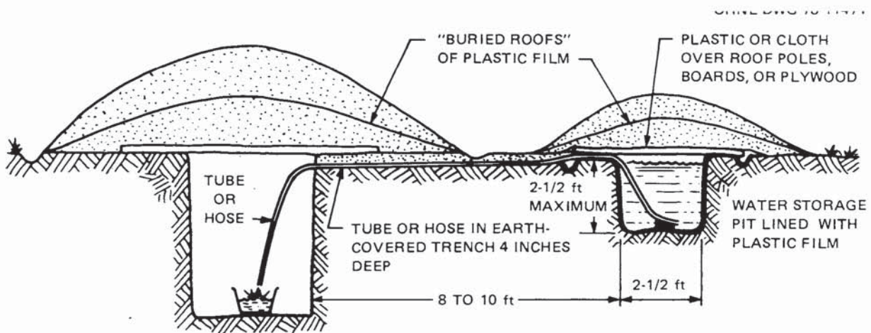
Fig. 8.7. Water siphoned into a belowground shelter.
