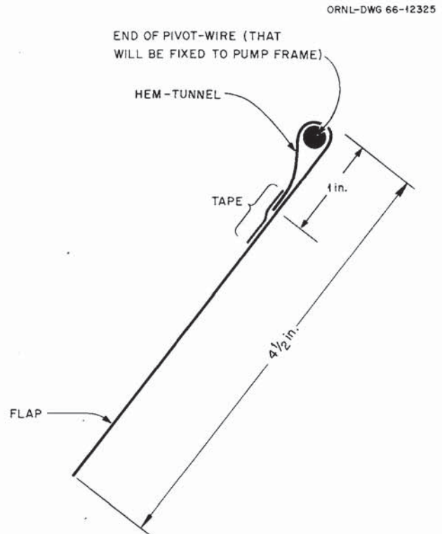
Fig. 7. End view.
