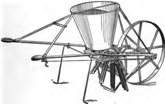
FIG. 12. WHEELBARROW FERTILIZER DISTRIBUTOR
