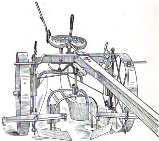
FIG. 77. CELERY HILLER
