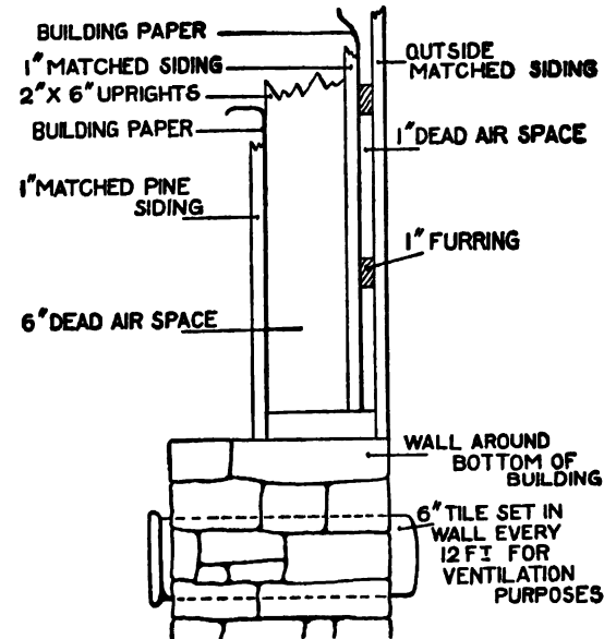
FIG. 70. NEW YORK CABBAGE HOUSE, SHOWING WALL CONSTRUCTION
