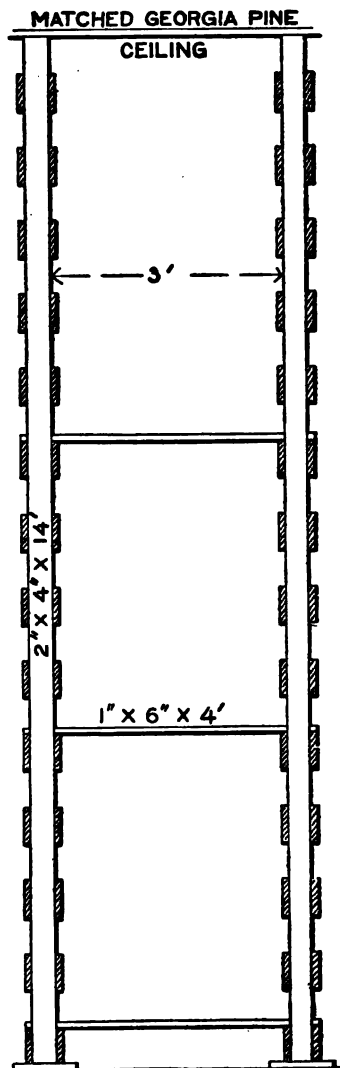
FIG. 71. NEW YORK CABBAGE HOUSE SHOWING BIN CONSTRUCTION
